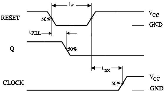
Figure 2. Switching Waveforms
