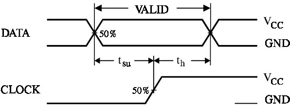
Figure 3. Switching Waveforms
