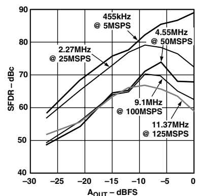
Figure 27. Single-Tone SFDR vs. A_{OUT} @ f_{OUT} = f_{CLOCK}/11
