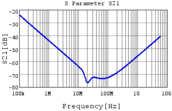
NFM18PS105D0J3 S21 DCOV,25degC, Feedthrough
