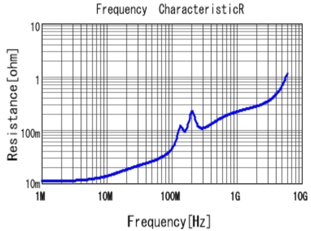
■ GRM1887U1A123JA01 R DCOV, 25degC
