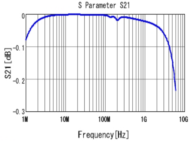
■ GRM1887U1A123JA01 S21 DCOV, 25degC
