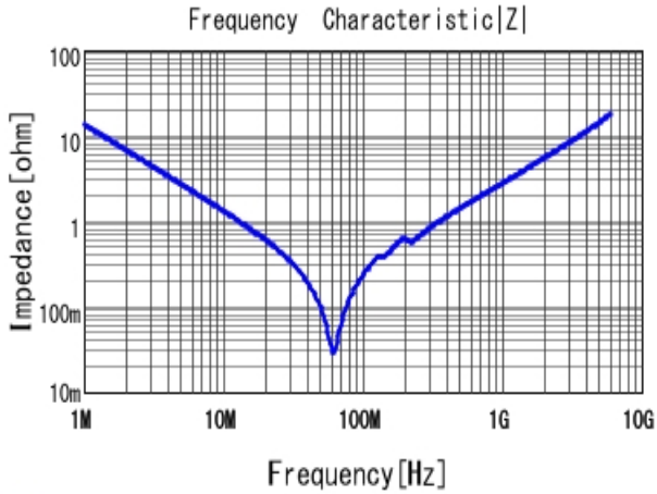
■ GRM1887U1A123JA01 |Z| DCOV, 25degC
