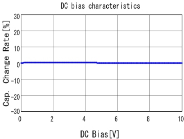
■ GRM1887U1A123JA01 C-DC bias capchange, 25.0degC, AC1V
