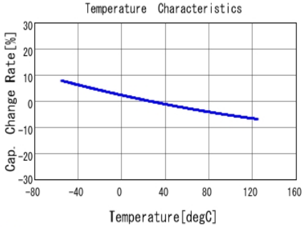
■ GRM1887U1A123JA01 C-Temp. capchange, DCOV, AC1Vrms
