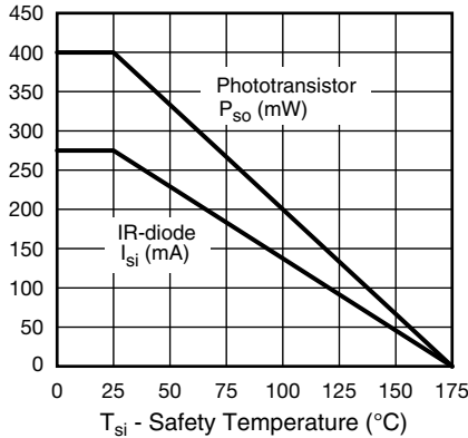
Fig. 1 - Derating Diagram
