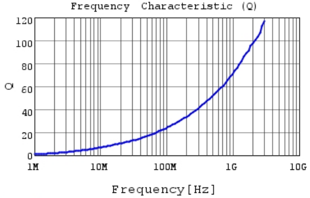
LQW15AN5N1G8Z Q
