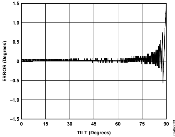
Figure 33. Inclusion Quantization Error
