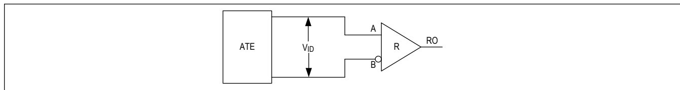
Figure 7. Receiver Propagation Delay Test Circuit
