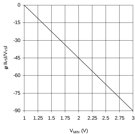
Graph 5. \phi I_{lvs}/V_{vsI} vs V_{MIN} (IR21592/IR21593)
