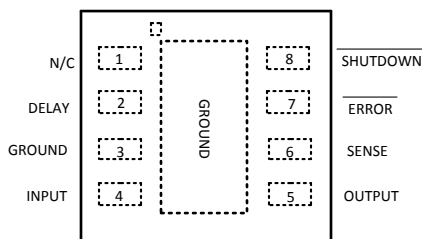
Figure 2. Top View 8-Lead WSON Surface Mount Package See Package Drawing Number NGN0008A
