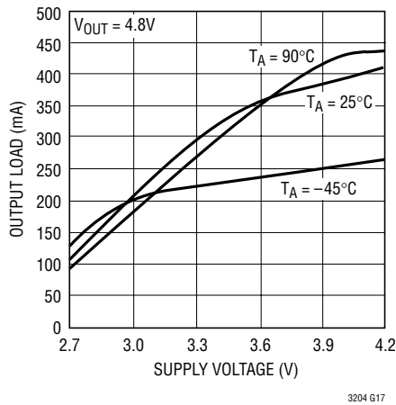
Output Load Capability at 4% Below Regulation
