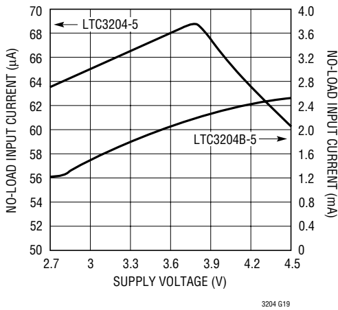
No-Load Input Current vs Supply Voltage
