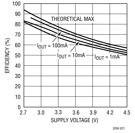
Efficiency vs Supply Voltage
