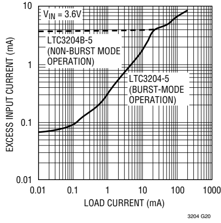
Extra Input Current vs Load Current ( I_{IN} - 2I_{LOAD} )
