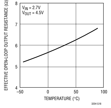
Effective Open-Loop Output Resistance vs Temperature
