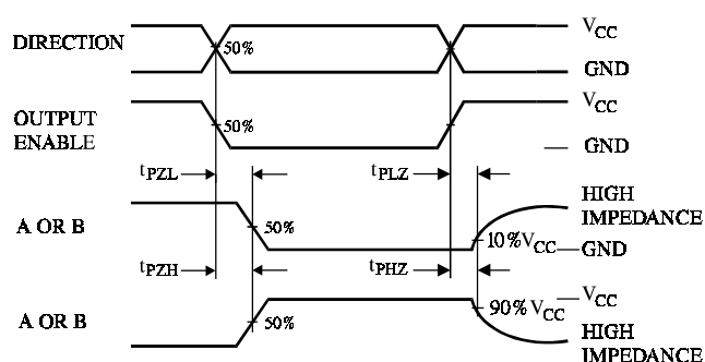
Figure 2. Switching Waveforms
