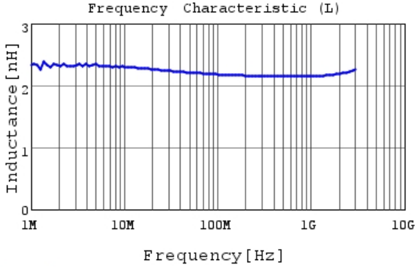
LQW15AN2N2G8Z L
