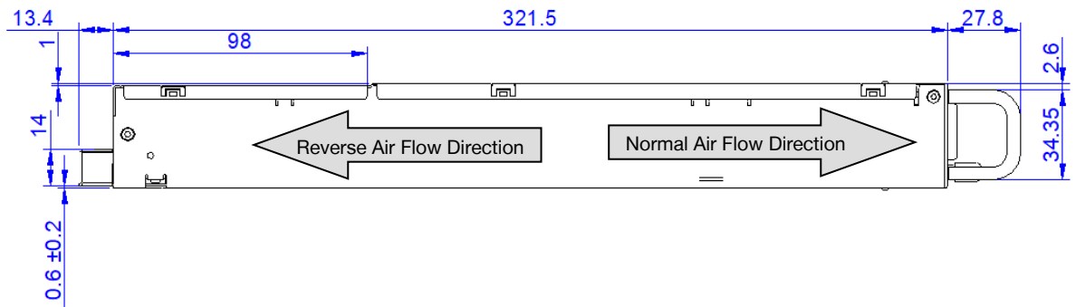
Figure 42. Side View 1
