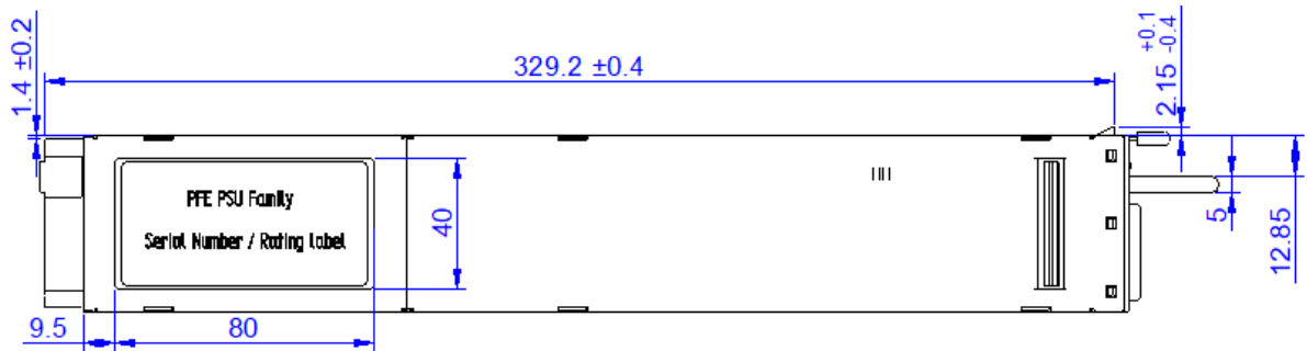
Figure 43. Top View
