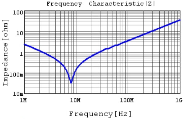
RDE5C1H683J2K1H03B |Z| DC0V, 25degC
