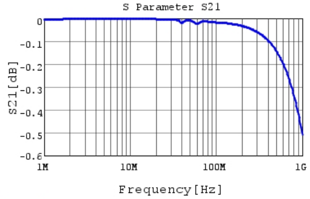
RDE5C1H683J2K1H03B S21 DCOV, 25degC
