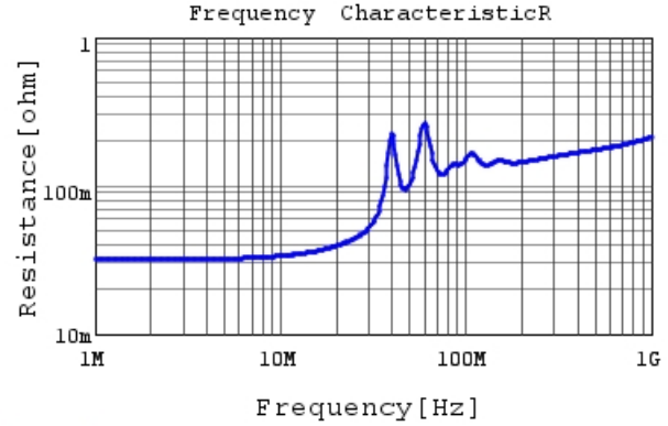
RDE5C1H683J2K1H03B R DC0V, 25degC
