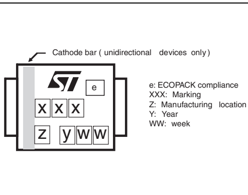
Figure 14. Marking layout (1)
