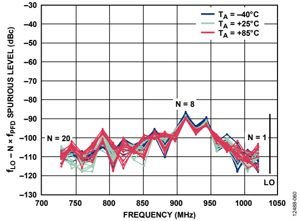
Figure 57. PFD Spurious Emissions on Modulator Output, f_{LO} - N \times f_{PFD} ; f_{LO} = 1036.8 MHz, R_{FOUT} = 4 dBm at 25°C, f_{REF} = 61.44 MHz at 4 dBm, f_{PFD} = 15.36 MHz, Integer PLL Mode
