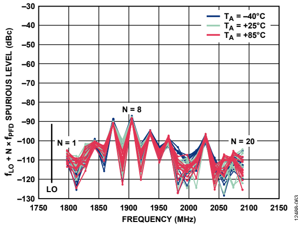
Figure 60. PFD Spurious Emissions on Modulator Output, f_{LO} + N \times f_{PFD} ; f_{LO} = 1781.76 MHz, R_{F_{OUT}} = 4 dBm at 25^{\circ}\text{C} , f_{REF} = 61.44 MHz at 4 dBm, f_{PFD} = 15.36 MHz, Integer PLL Mode
