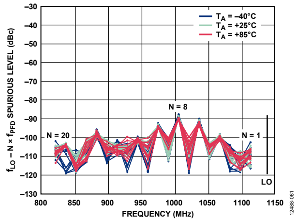
Figure 58. PFD Spurious Emissions on Modulator Output, f_{LO} - N \times f_{PFD} ; f_{LO} = 1128.96 MHz, R_{FOUT} = 4 dBm at 25°C, f_{REF} = 61.44 MHz at 4 dBm, f_{PFD} = 15.36 MHz, Integer PLL Mode
