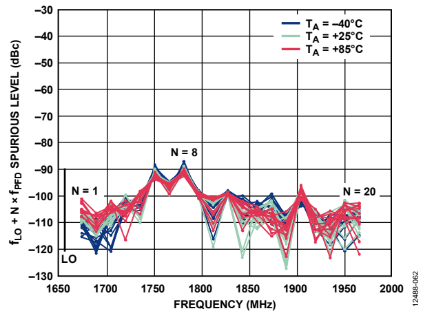
Figure 59. PFD Spurious Emissions on Modulator Output, f_{LO} + N \times f_{PFD} ; f_{LO} = 1658.88 MHz, R_{FOUT} = 4 dBm at 25°C, f_{REF} = 61.44 MHz at 4 dBm, f_{PFD} = 15.36 MHz, Integer PLL Mode
