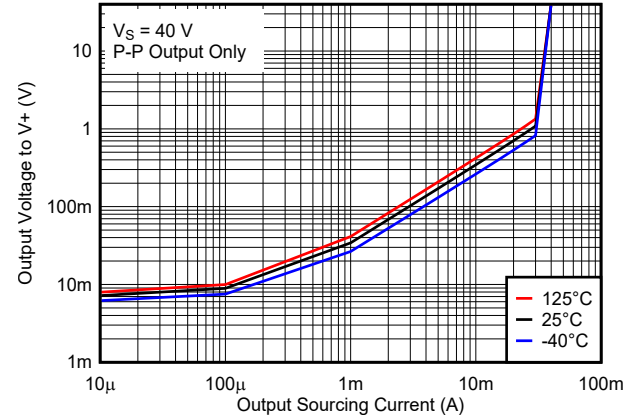
Figure 7-10. Output Voltage vs. Output Sourcing Current, 40 V
