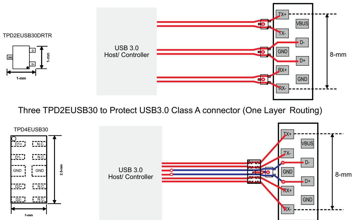
One TPD4EUSB30 & One TPD2EUSB30 to Protect USB3.0 Class A connector (Two Layer Routing)
