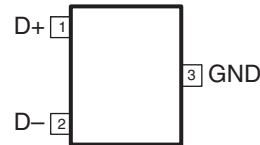
DQA PACKAGE (TOP VIEW)
