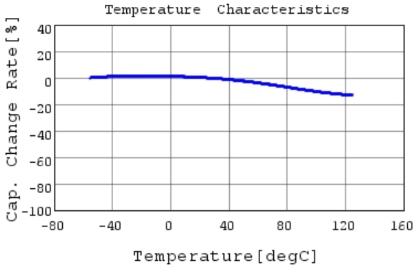
GRM31MR71E225KA93 C-Temp. capchange, DC0.0V,
