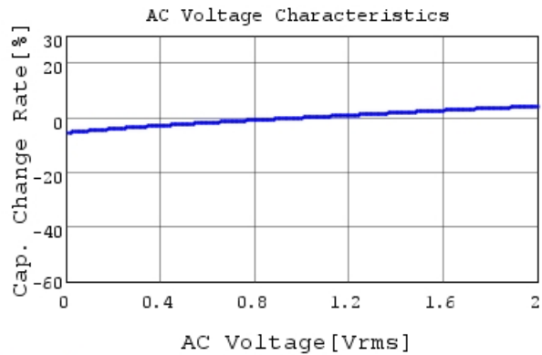
GRM31MR71E225KA93 C-AC Voltage capchange, Dc
