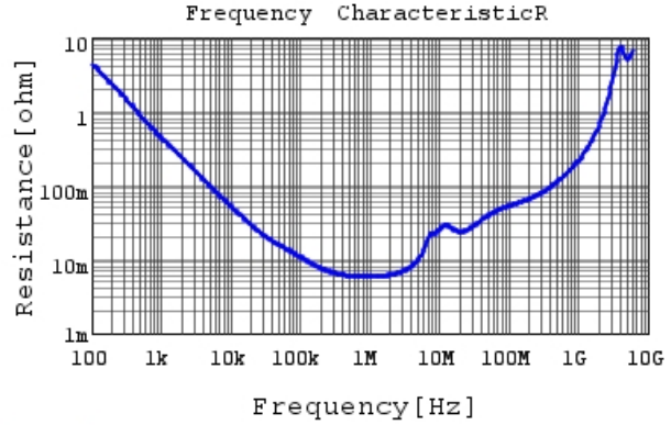
GRM31MR71E225KA93 R DCOV, 25degC
