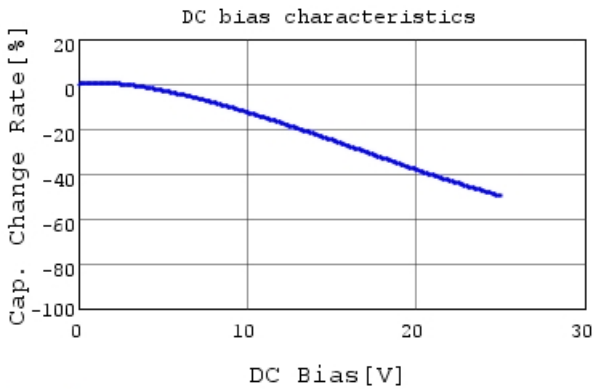
GRM31MR71E225KA93 C-DC bias capchange, 25.0c
