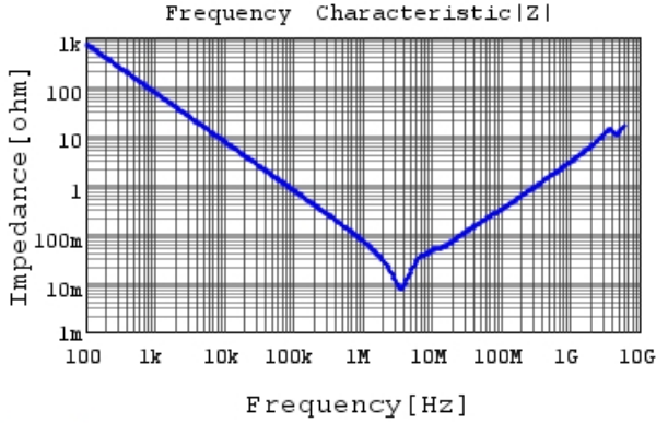
GRM31MR71E225KA93 |Z| DCOV, 25degC
