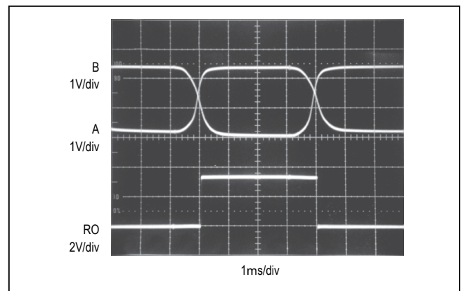
Figure 18. MAX3483/MAX3488 Receiver Propagation Delay
