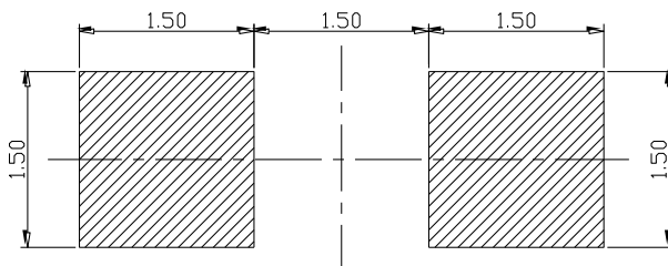
Recommended Soldering Pad
