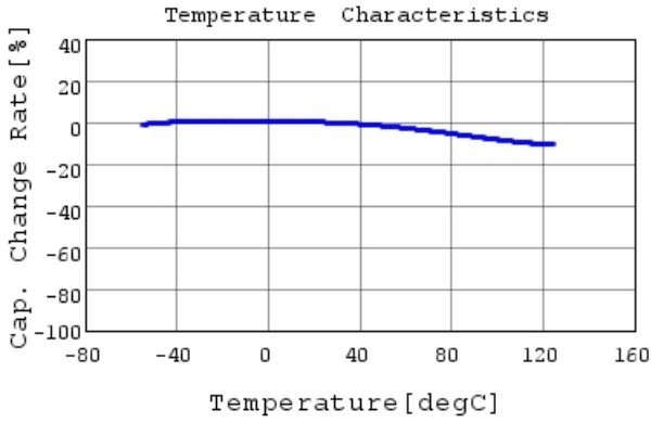
GRM31CR71H225KA88 C-Temp. capchange, DC0.0V,
