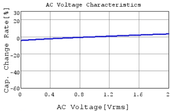
GRM31CR71H225KA88 C-AC Voltage capchange, D
