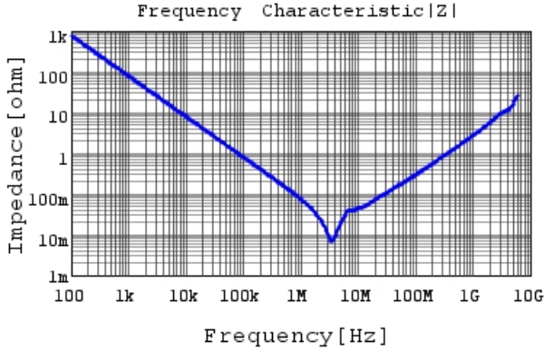
GRM31CR71H225KA88 |Z| DCOV, 25degC
