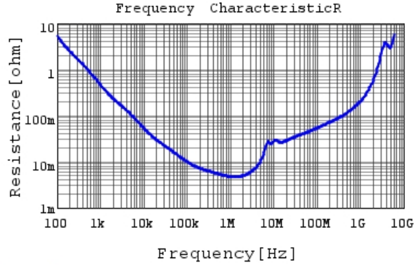
GRM31CR71H225KA88 R DCOV, 25degC
