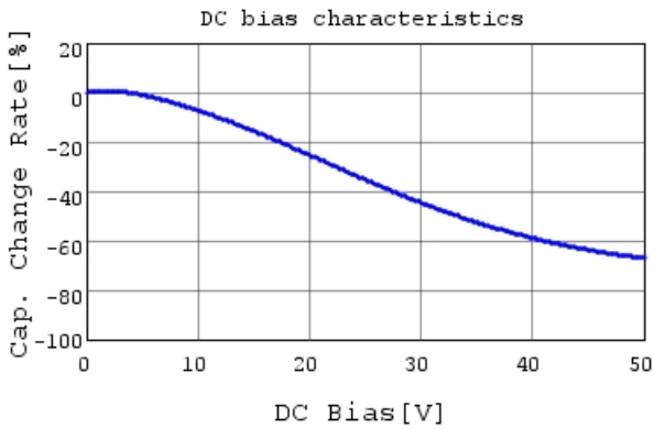
GRM31CR71H225KA88 C-DC bias capchange, 25.0c
