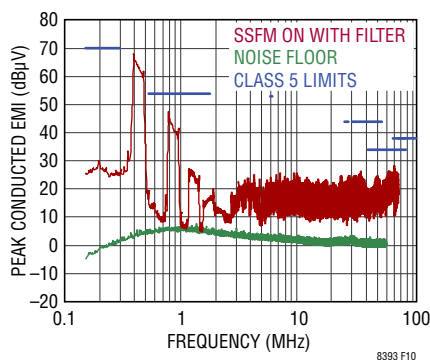
Figure 10. CISPR 25 Peak Conducted EMI
