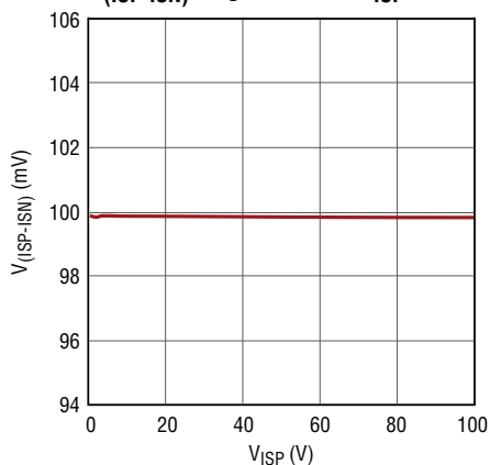
V_{(ISP-ISN)} Regulation vs V_{ISP}
