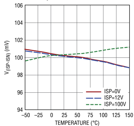
V_{(ISP-ISN)} Regulation vs Temperature
