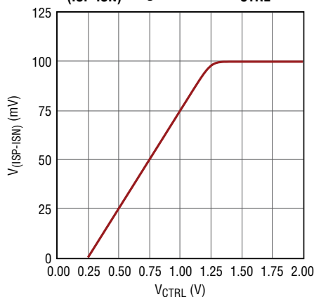
V_{(ISP-ISN)} Regulation vs V_{CTRL}
